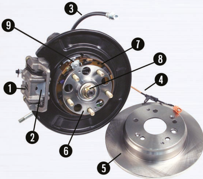
Rear Disc Brake Assembly
