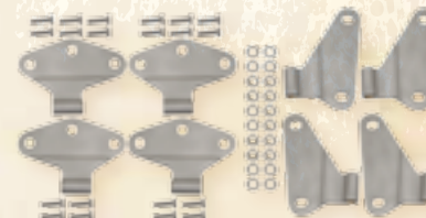
40581 Body Door Hinge Set (8 pieces) (4 door) Fits: JK - 2007-Up Finish: Sand Blasted Ready to Paint Stainless Steel
