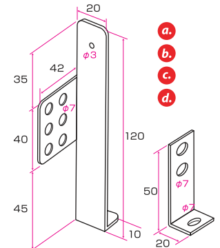
Brackets for Street Oil Catch Tank
