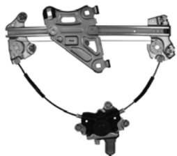
88964 G88964 ACI Plus Power Window Motor and Regulator Assembly Kia (14-10) Kia: 824011M200
