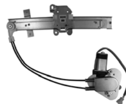
88045 D88045 ACI Plus Power Window Motor and Regulator Assembly Mazda (98-95)
