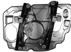
384312 Z384312 ACI Plus Power Window Regulator Ford (09-05); Mercury (09-05) Ford: 8G1Z5423209B
