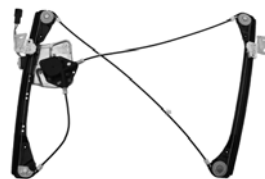
82111 E82111 ACI Plus Power Window Motor and Regulator Assembly Olds (04-99); Pontiac (05-99)
