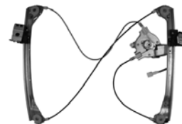
389003 G389003 ACI Plus Power Window Motor and Regulator Assembly BMW (06-00) BMW: 51338229106
