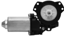
389489 A389489 ACI Plus Power Window Motor General Motors Corp: 19297737, 19297766, 19297769, 19297770, 19297773 Hyundai: 834503K001
