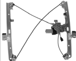
82122 H82122 ACI Plus Power Window Motor and Regulator Assembly Cadillac (06-02); Chevy (07-99); GMC (07-99) General Motors Corp: 19120847
