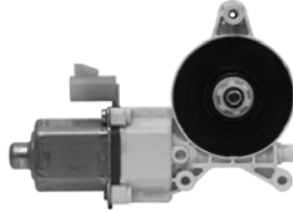
82284 B82284 ACI Plus Power Window Motor Cadillac (14-08)
