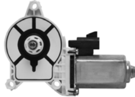
82987 B82987 ACI Plus Power Window Motor Buick (11-06); Chevy (10-05); Pontiac (09-06) General Motors Corp: 15929736
