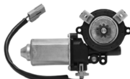
83128 B83128 ACI Plus Power Window Motor Ford (11-93); Mazda (10-94); Mercury (07-04) Ford: 6F2Z7823395BA, 8L5Z7823395A
