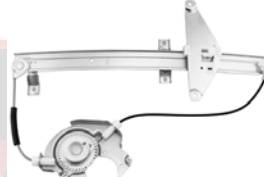
81889 D81889 ACI Plus Power Window Regulator Honda (97-94); Isuzu (97-94) Honda: 8971658802
