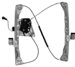
82312 K82312 ACI Plus Power Window Motor and Regulator Assembly Buick (07-02); Pontiac (05-01) General Motors Corp: 15911244
