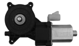
382365 A382365 ACI Plus Power Window Motor Cadillac (12-10); Chevy (13-10); GMC (11-10) General Motors Corp: 25909231, 96964419, 96964422
