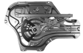
88960 Z88960 ACI Plus Power Window Motor and Regulator Assembly Kia (09-07) Kia: 824013F020
