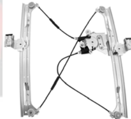
81279 H81279 ACI Plus Power Window Regulator Buick (07-04); Chevy (09-02); GMC (09-02); Isuzu (08-03); Olds (04-02); Saab (09-05) General Motors Corp: 19331461
