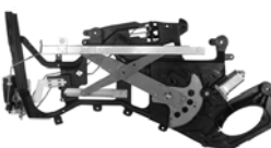
382345 Z382345 ACI Plus Power Window Motor and Regulator Assembly Chevy (05-97); Olds (99-97) General Motors Corp: 22723562
