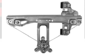
384713 E384713 ACI Plus Manual Window Regulator Chevy (16-12) General Motors Corp: 95494531
