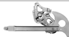
81249 D81249 ACI Plus Power Window Regulator Chevy (94-82); GMC (94-82); Olds (94-91) General Motors Corp: 19251095
