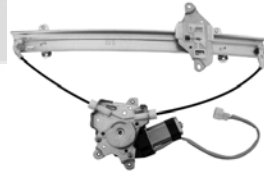
88416 D88416 ACI Plus Power Window Motor and Regulator Assembly Mitsubishi (03-02)
