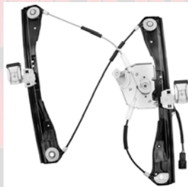
82233 H82233 ACI Plus Power Window Motor and Regulator Assembly Pontiac (10-05) General Motors Corp: 25931990
