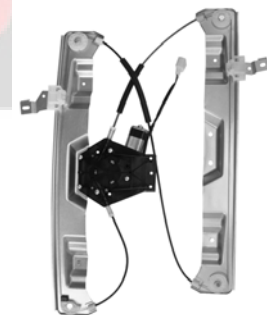
83156 H83156 ACI Plus Power Window Motor and Regulator Assembly Ford (09-02); Mercury (09-02) Ford: 6L2Z7823201BA
