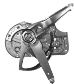
384966 E384966 ACI Plus Power Window Regulator Volvo (14-03)
