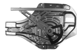
384999 Z384999 ACI Plus Power Window Regulator Hyundai (09-05) Hyundai: 824062E000
