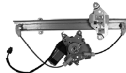
88293 D88293 ACI Plus Power Window Motor and Regulator Assembly Nissan (15-05)
