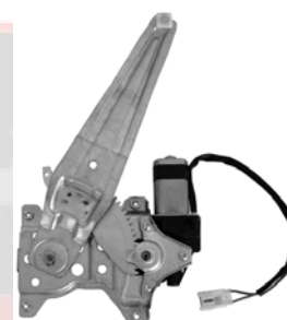
88722 D88722 ACI Plus Power Window Motor and Regulator Assembly Toyota (14-07)
