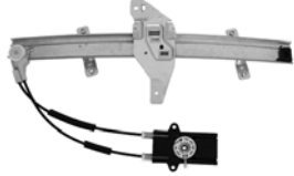
81220 E81220 ACI Plus Power Window Regulator Buick (05-97); Olds (02-98)
