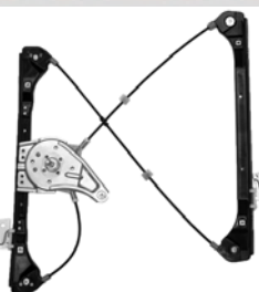
81919 E81919 ACI Plus Manual Window Regulator Olds (04-99); Pontiac (05-99) General Motors Corp: 22697442
