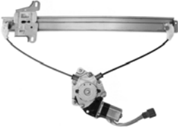
389095 K389095 ACI Plus Power Window Motor and Regulator Assembly Acura (12-05)
