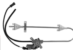
389084 D389084 ACI Plus Power Window Motor and Regulator Assembly Kenworth (10-03); Peterbilt (10-06)
