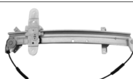
81306 H81306 ACI Plus Power Window Regulator Ford (11-92); Mercury (11-92) Ford: 6W7Z5427009AA
