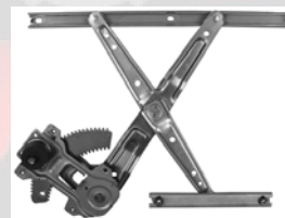
81049 D81049 ACI Plus Manual Window Regulator Hyundai (89-86); Mitsubishi (89-87) Hyundai: 8340221001
